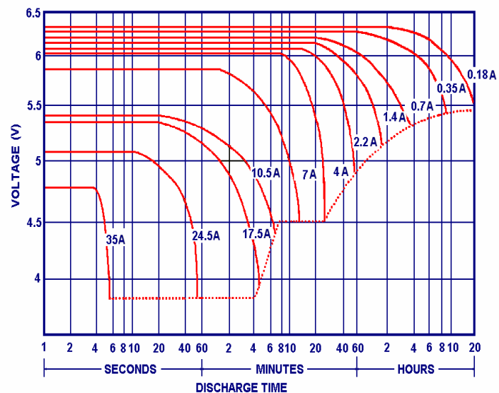
DISCHARGE CHARACTERISTIC CURVE
